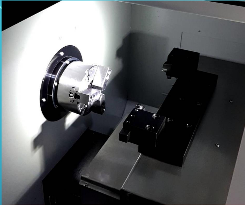
CLAMP: 5"
